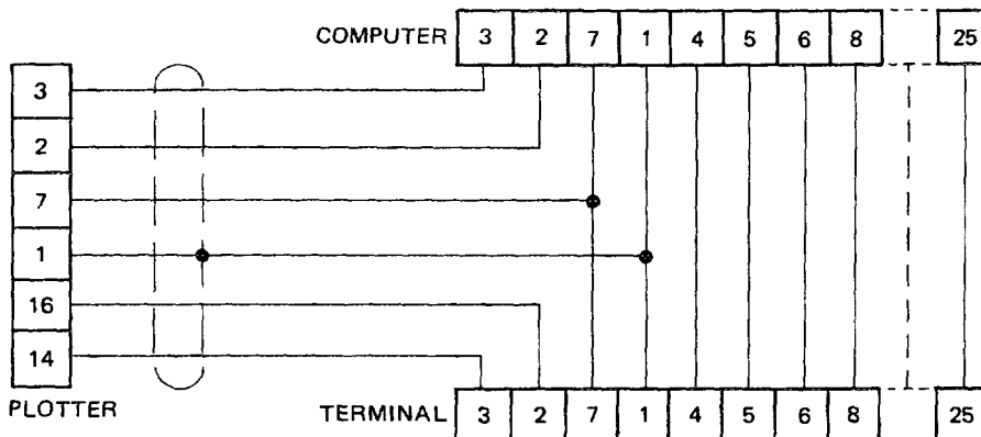
PINS 4, 5, 6, AND 8 THROUGH 25 ARE DIRECTLY CONNECTED BETWEEN THE COMPUTER AND TERMINAL CONNECTORS.
